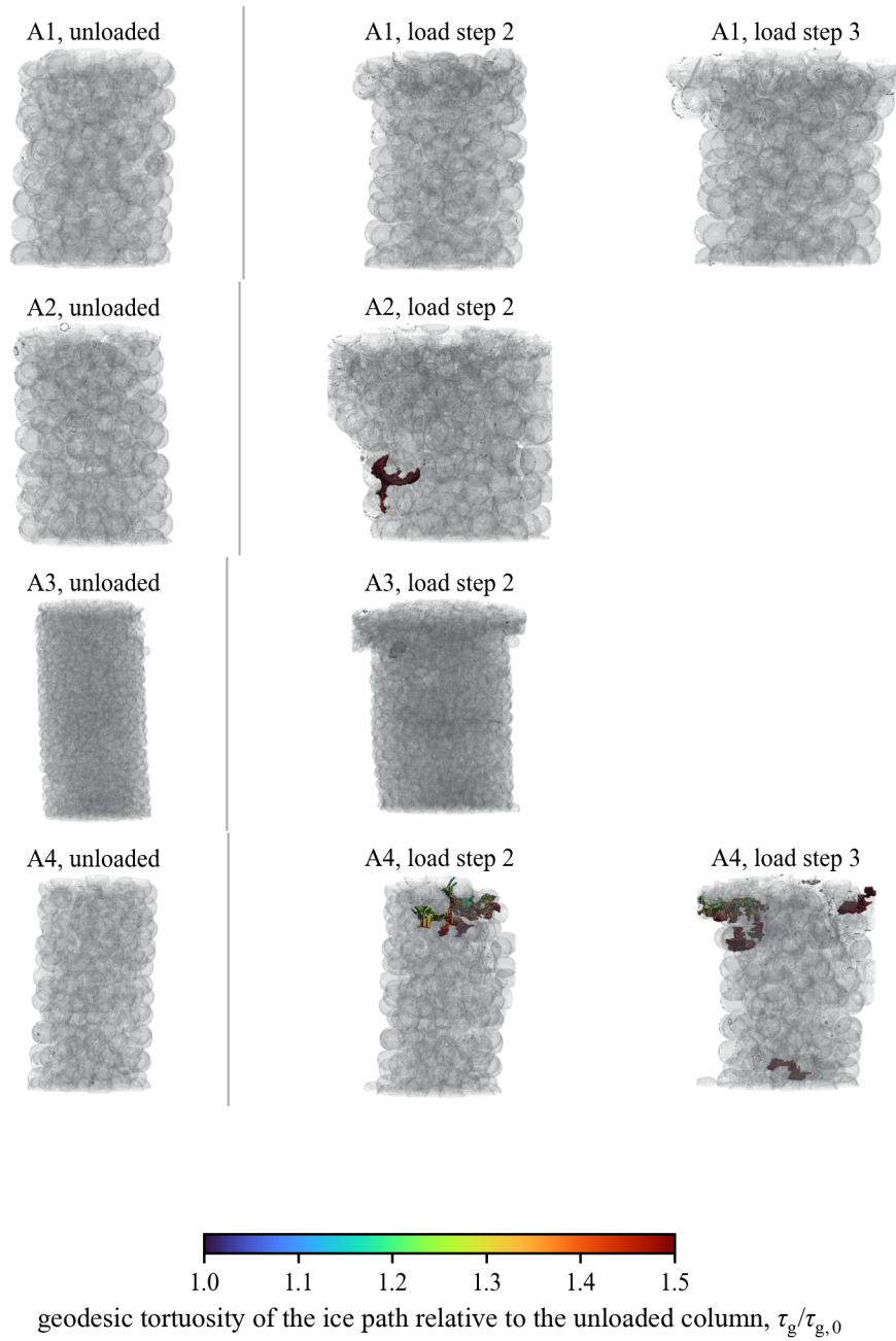
Figure S6: Ice-path maps of the \gamma -alumina specimens.
