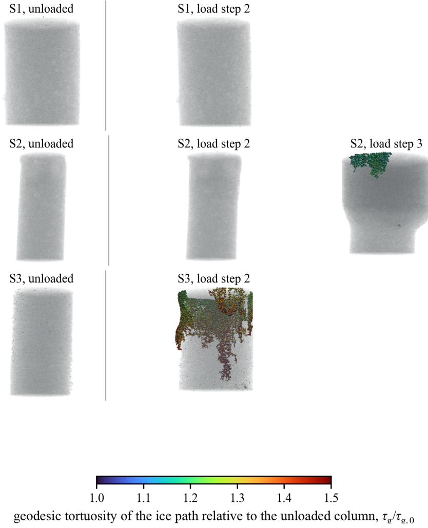
Figure S7: Ice-path maps of the sand specimens.
