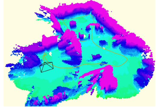
Fig. 10. Experiments in an indoor scene composed of two rooms: a small one with tables and chairs (top left), a large room cluttered with obstacles (top right).
