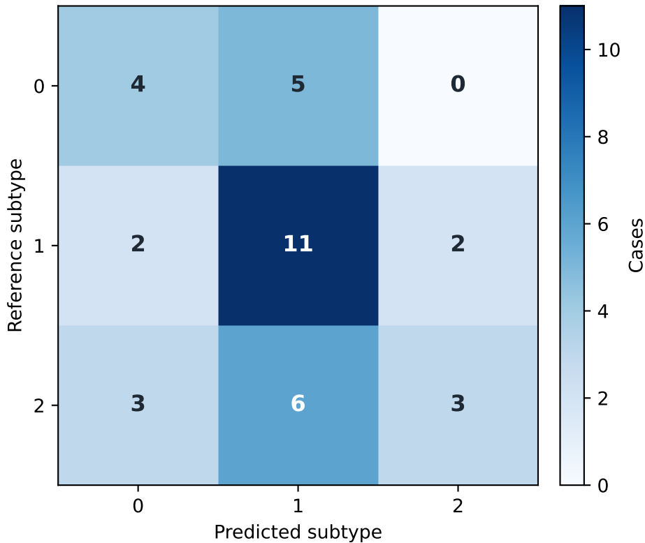
Validation confusion matrix (n=36)
