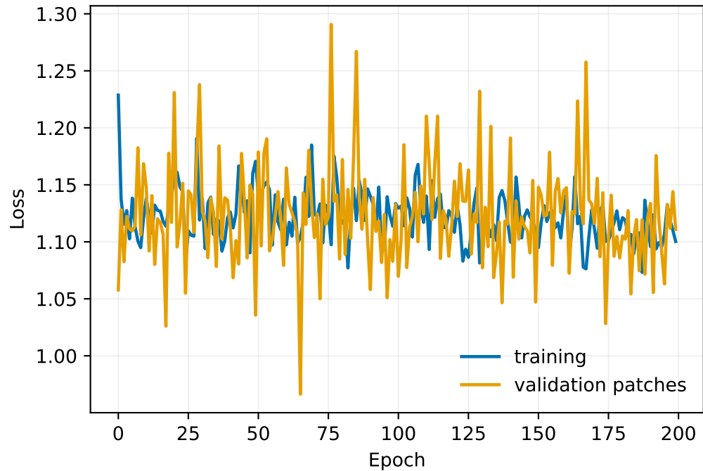
Classification objective
