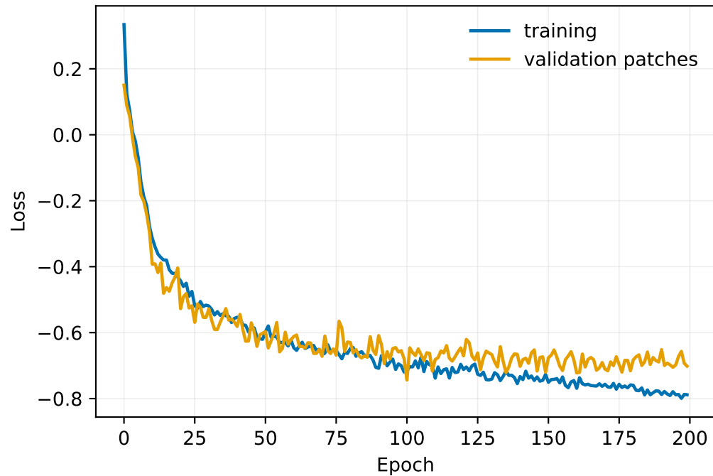
Segmentation objective
