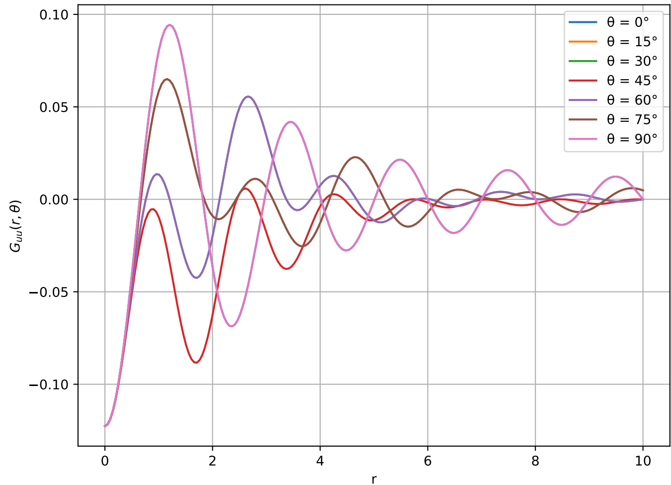
Normal Green's Function in Polar Coordinates
