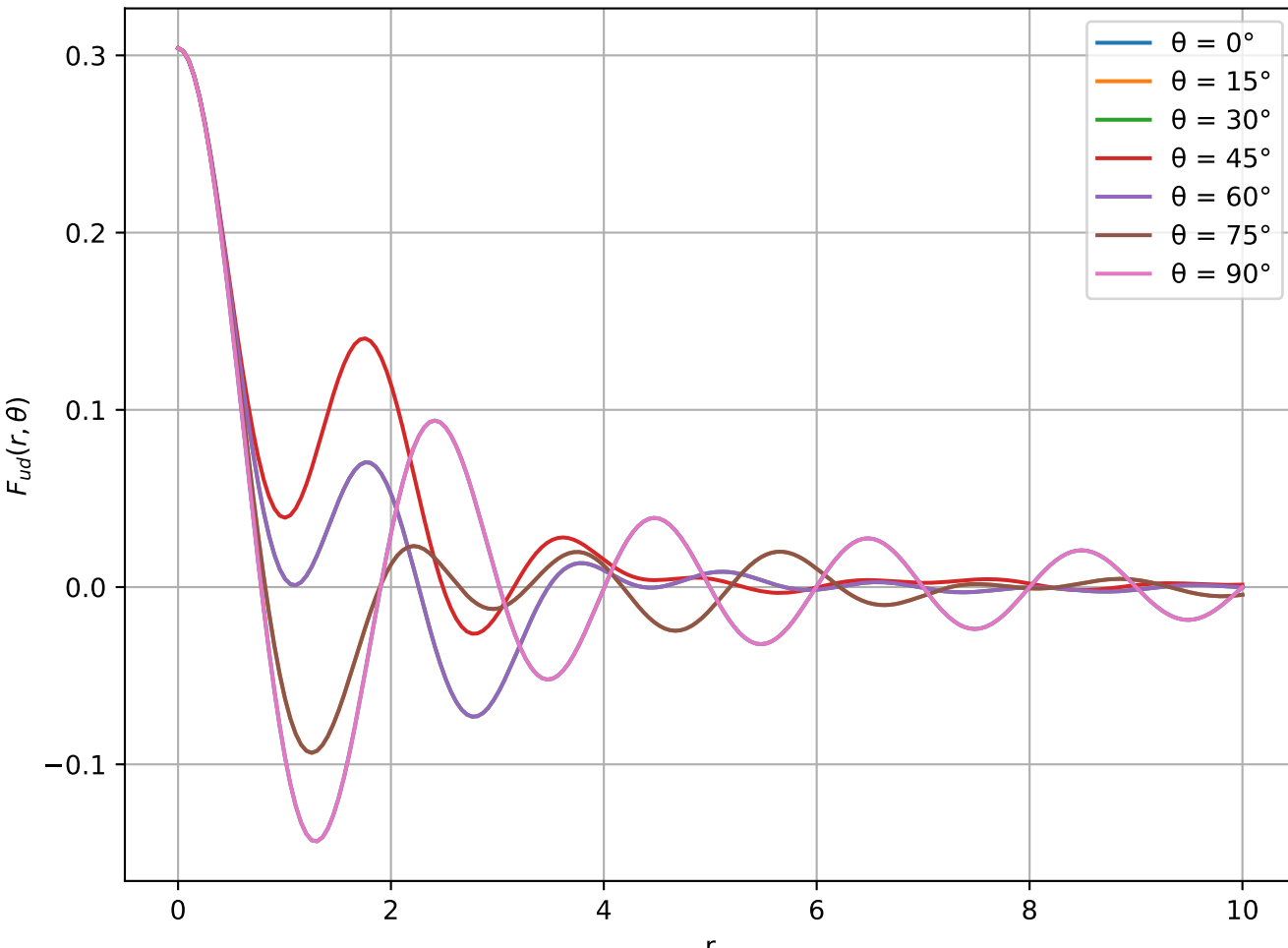
Anomalous Green's Function in Polar Coordinates
