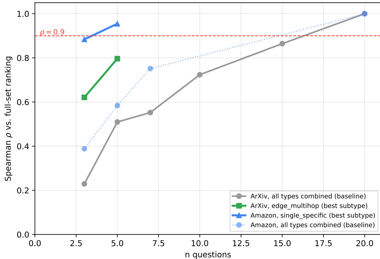
GraphRAG: variant-ranking \rho vs. n questions (Study B/C not run -- gate not met, see caption)
