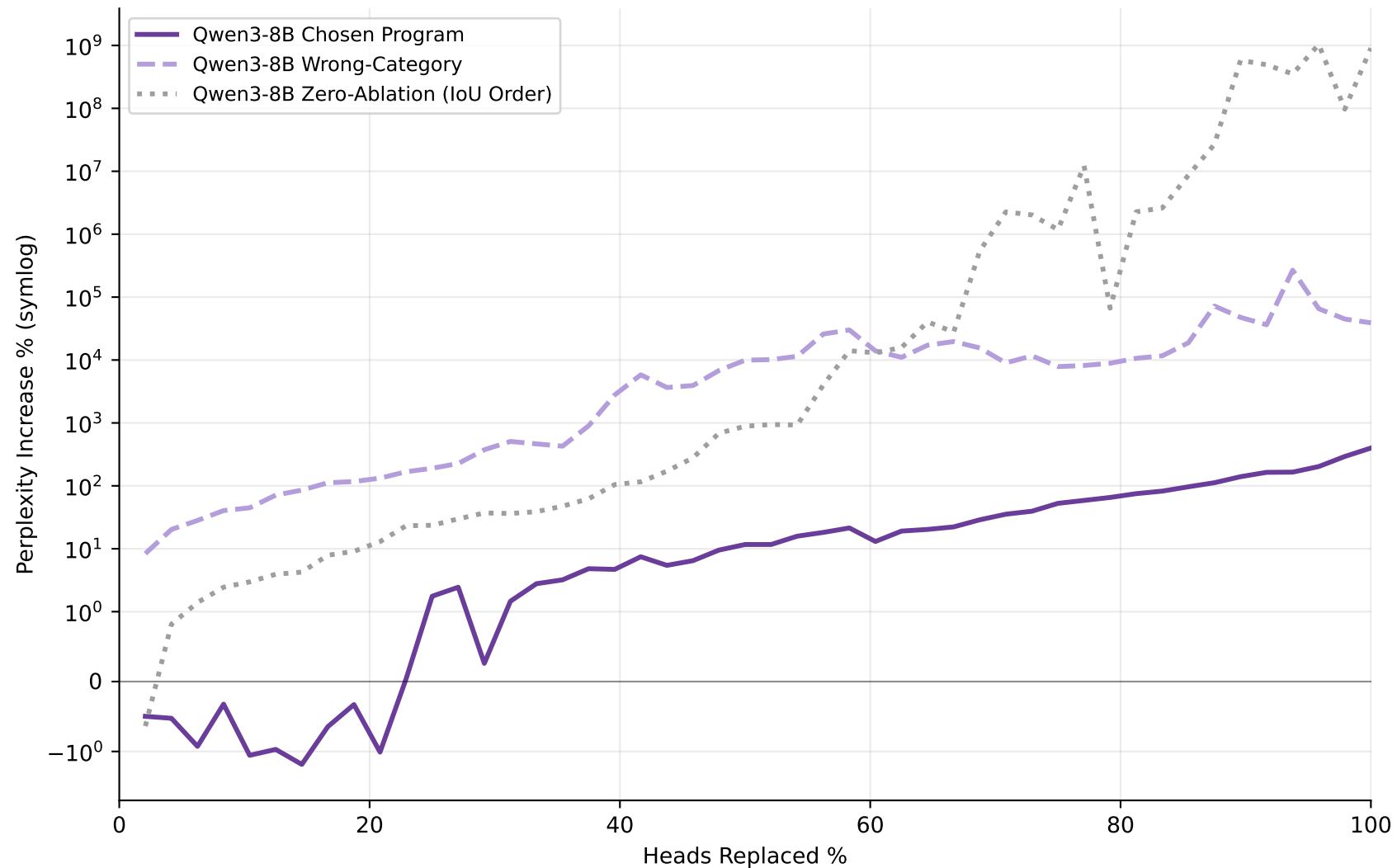
Head Replacement vs. Perplexity Increase — Qwen3-8B-Base
