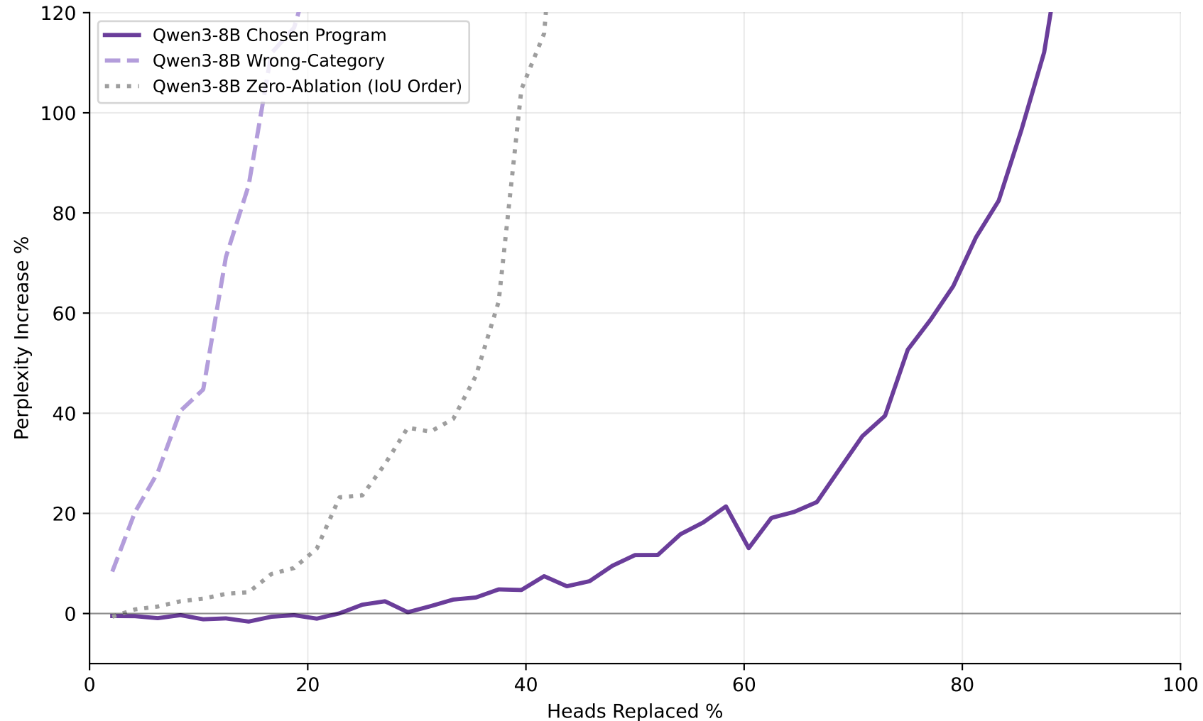
Head Replacement vs. Perplexity Increase — Qwen3-8B-Base (linear, clipped to +120% to show the chosen-program regime)
