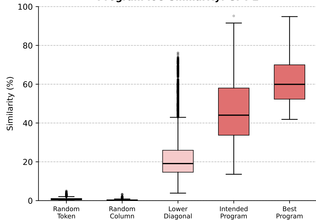
Program IoU Similarity: GPT-2
