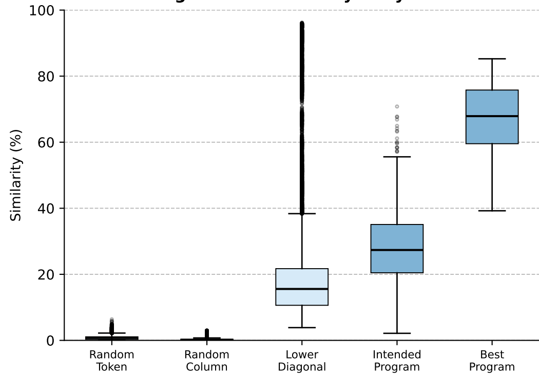
Program IoU Similarity: TinyLlama
