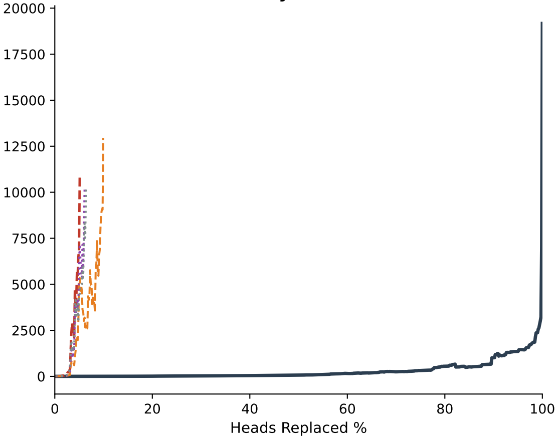
TinyLlama
