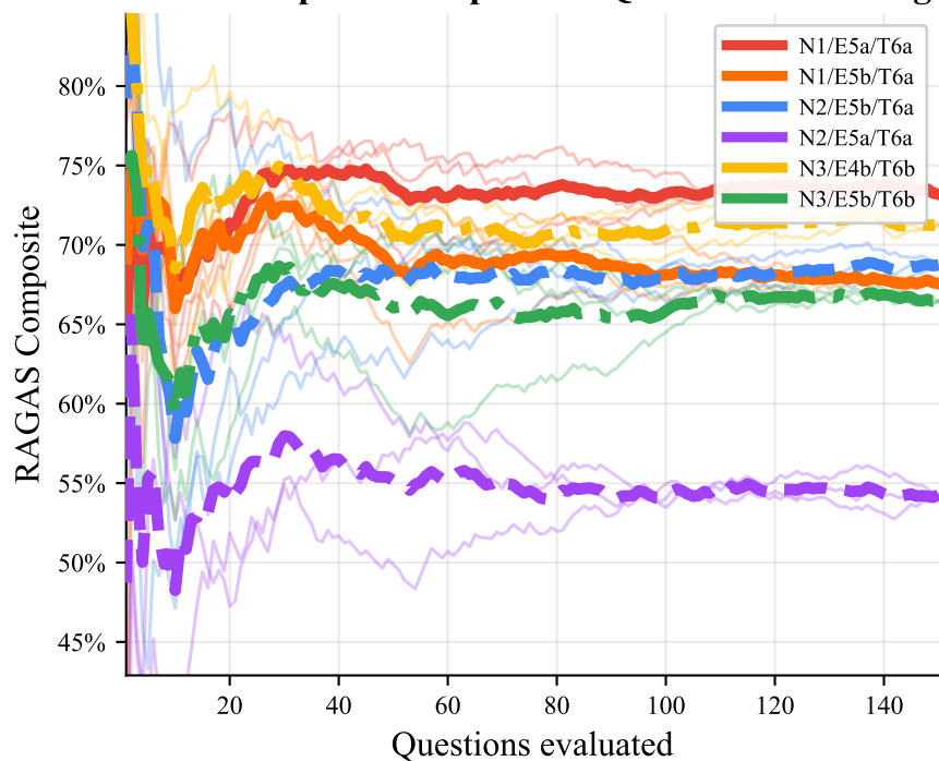
Amazon Sports: GraphRAG Question Answering
