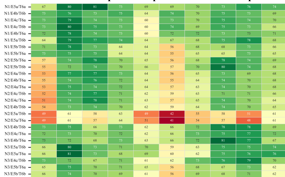
Amazon Sports: GraphRAG Score Heatmap
