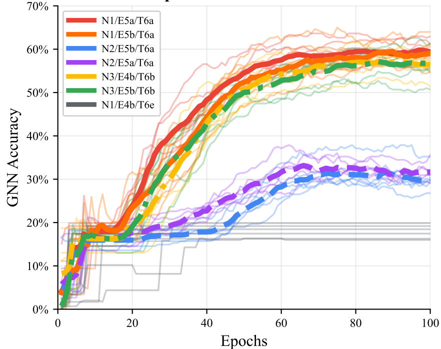
Amazon Sports: GNN Node Classification
