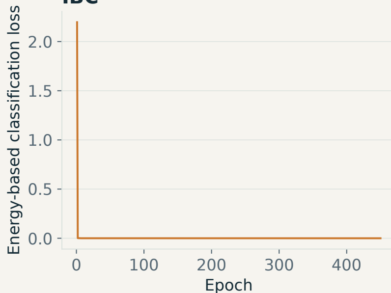
IBC
