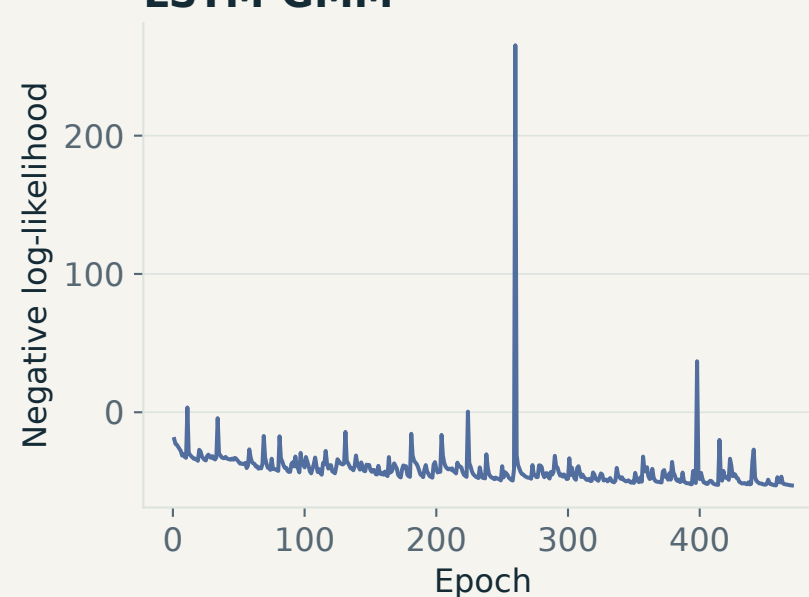
LSTM-GMM
