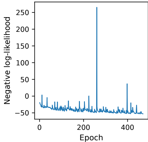
(c) LSTM-GMM
