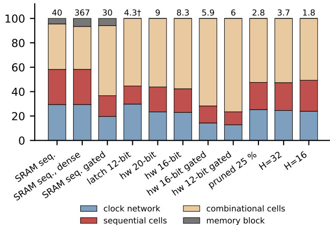
share of decode-time power (%)
