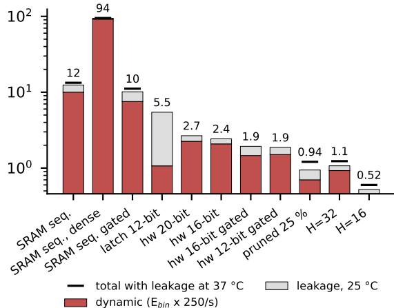
average power at 250 bins/s ( \mu\text{W} )
