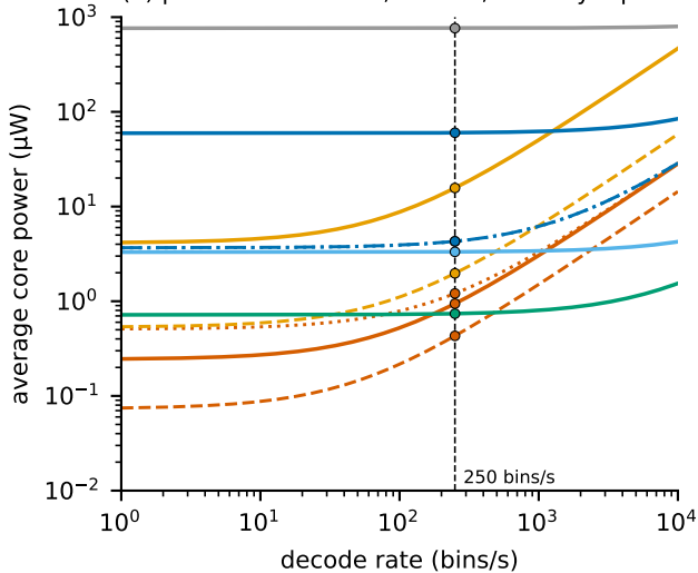
(a) pruned 12-bit core, H = 64 , 25 % synapses
