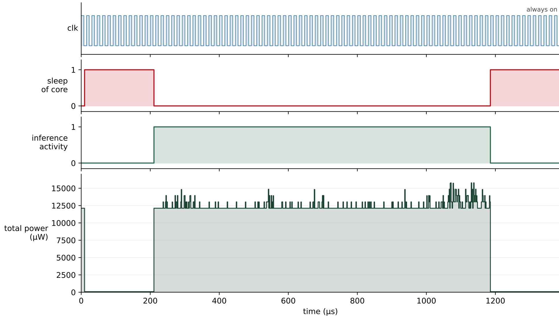
sky130 VexRiscv SoC — sleep / MNIST inference / time-based power
