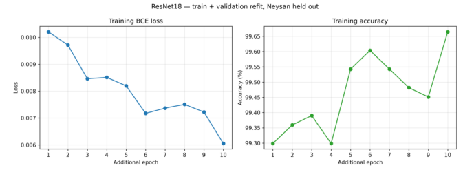
Figure 13. Supplied phase-two fixed-budget refit history. Training loss fell from 0.010207 to 0.006054. Final sampled training accuracy was 99.66%.
