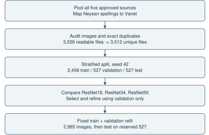
Figure 1. Phase-one workflow. The final test set is reserved during architecture comparison and validation experiments.
