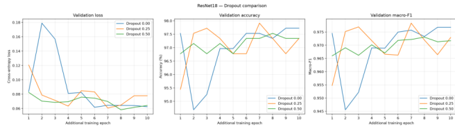
Figure 5. Dropout comparison. Dropout 0.25 was selected; dropout 0.50 did not improve on its initial checkpoint.
