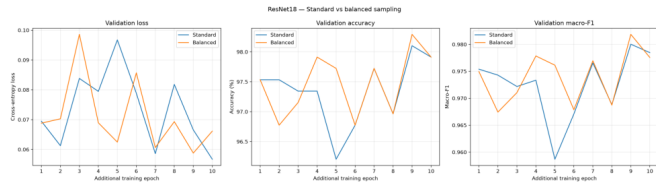
Figure 6. Standard versus balanced sampling. Balanced batches contained two images per class, for 16 images per batch.
