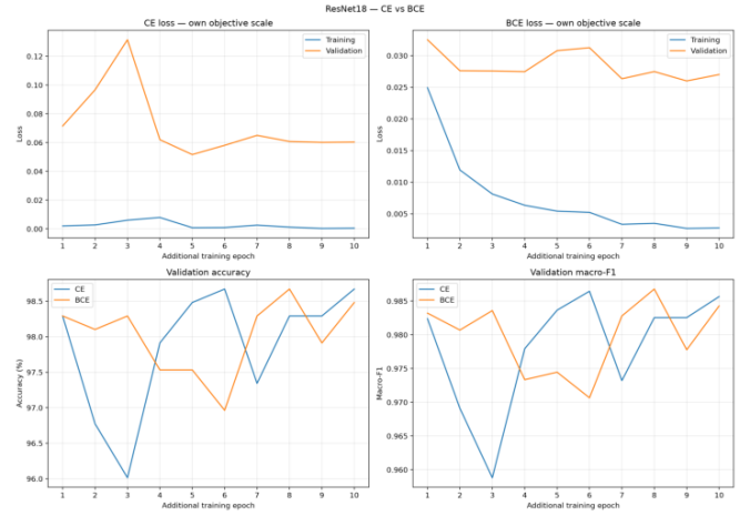
Figure 7. Supplied CE-versus-BCE comparison. The two losses have different scales and should not be ranked by their raw loss values.
