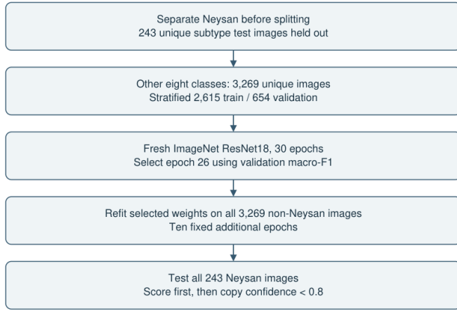
Figure 11. Neysan-holdout workflow. Phase-one vehicle-trained checkpoints were not reused because they had already seen Neysan.
