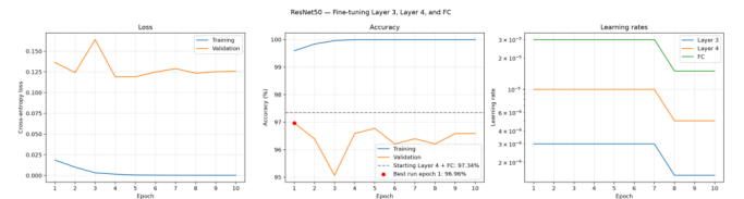
Figure 4. Supplied ResNet50 layer3+layer4 history. The retained 97.34% checkpoint came from the preceding layer4 stage.
