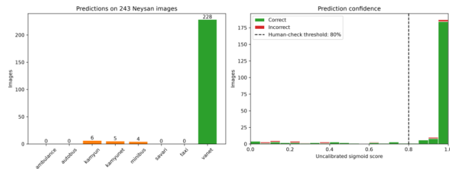
Figure 15. Supplied prediction-count and confidence-distribution summary for the Neysan test.
