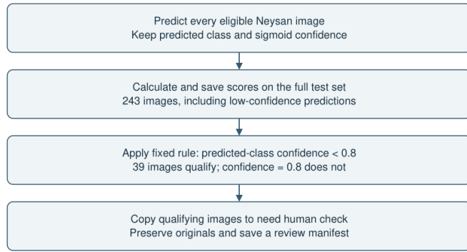
Figure 14. Review routing occurs after scoring. The confidence threshold does not remove difficult images from the reported test denominator.
