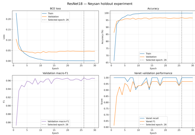
Figure 12. Supplied phase-two training curves, including Vanet validation recall and F1. The selected checkpoint was epoch 26.
