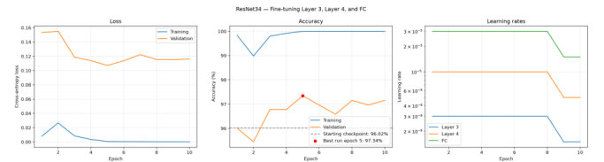
Figure 3. Supplied ResNet34 layer3+layer4 history. The best checkpoint in this stage was epoch 5, with 97.34% validation accuracy.
