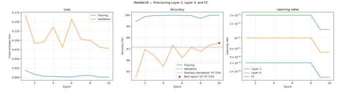
Figure 2. Supplied ResNet18 layer3+layer4 training history. The selected stage epoch was 10.
