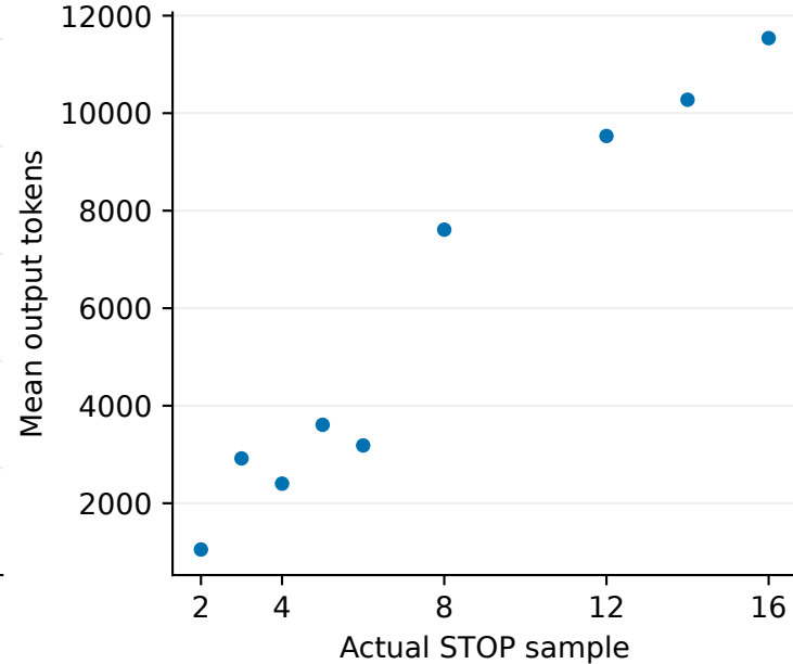
Stopping-conditioned outcomes and cost · descriptive
