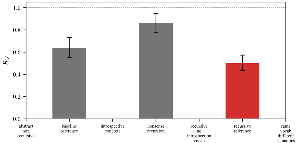
Circularity Controls: Structure vs Semantics
