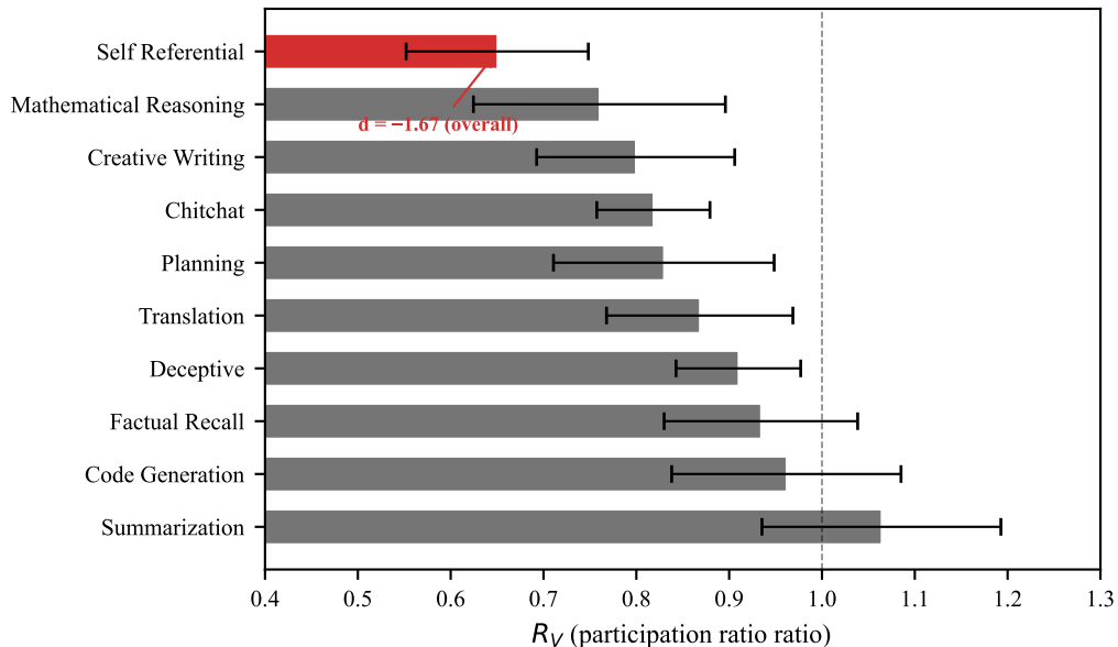
R_V Spectral Fingerprint Across 10 Computational Modes
