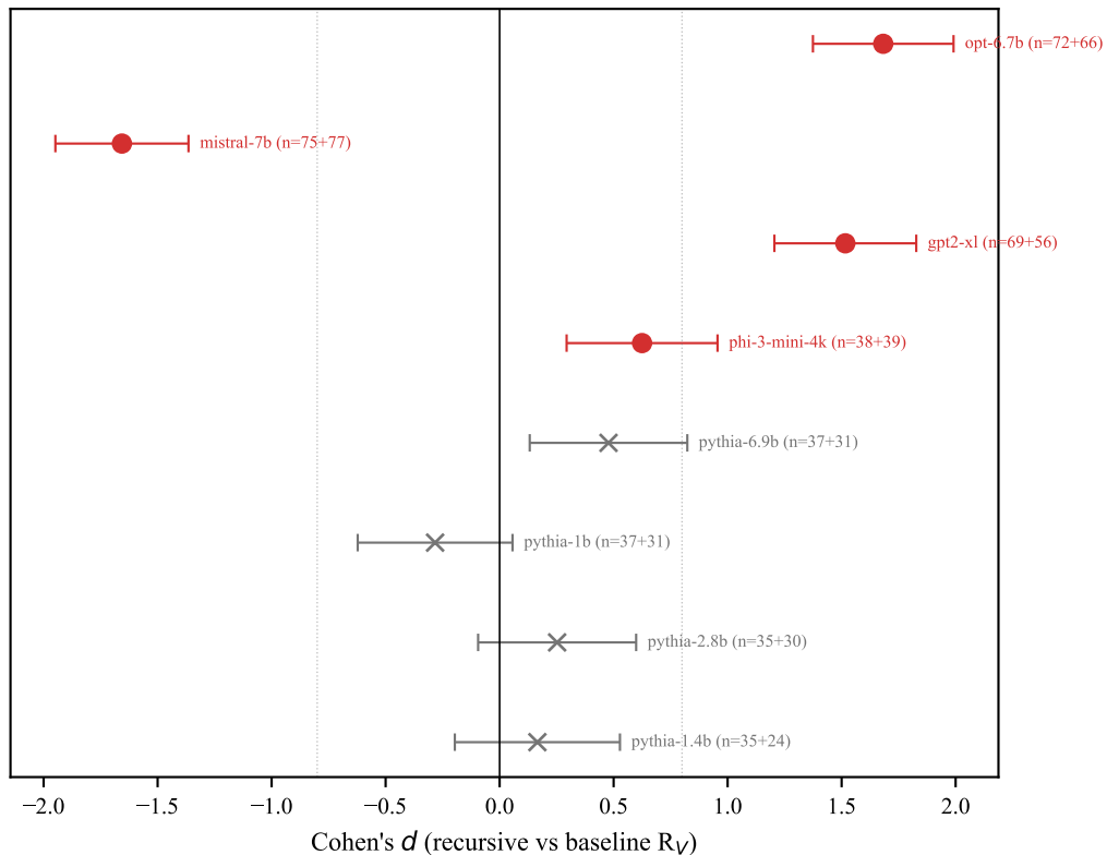
Cross-Architecture Forest Plot (8 models)
