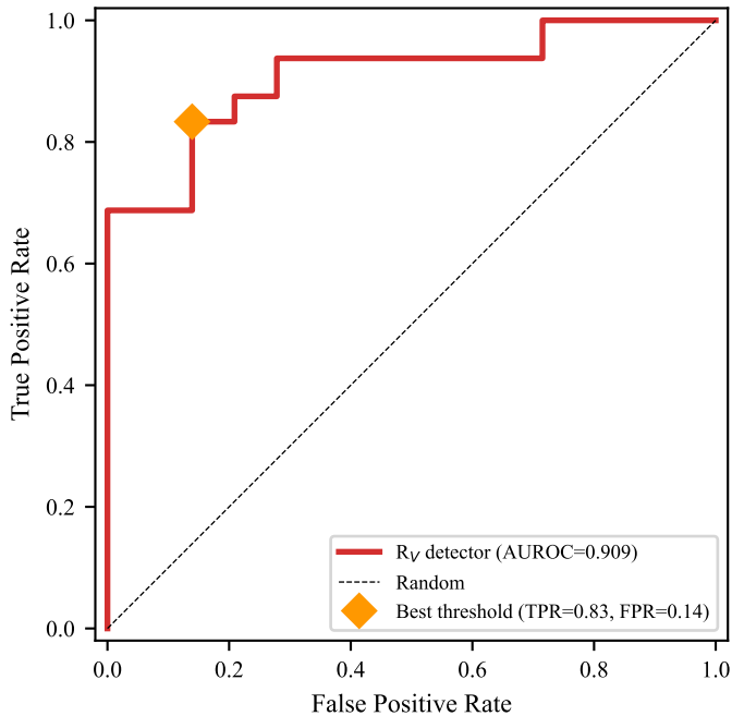
R_V -Based Self-Referential Processing Detector (500 prompts, 50 self-ref seeded)
