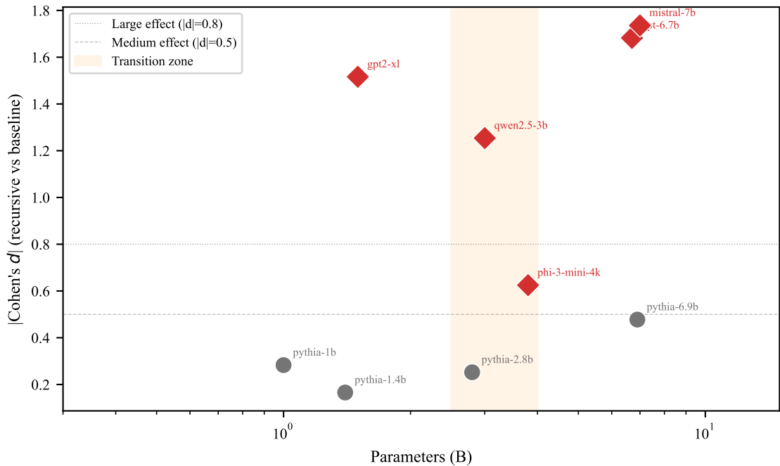
R_V Effect Size vs Model Scale (9 architectures, \square = p < 0.05 )
