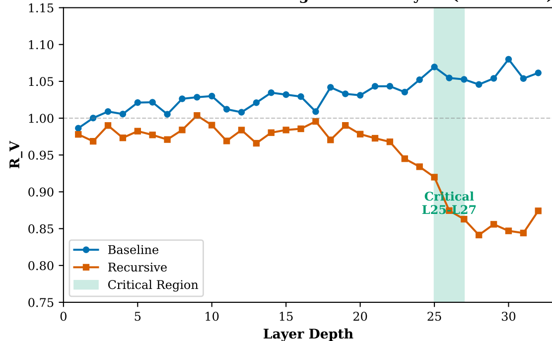
Geometric Contraction Emerges in Late Layers (Mistral-7B)
