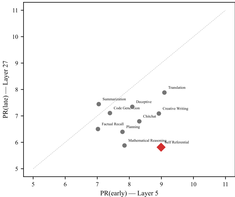
Spectral Fingerprint: Early vs Late Participation Ratio
