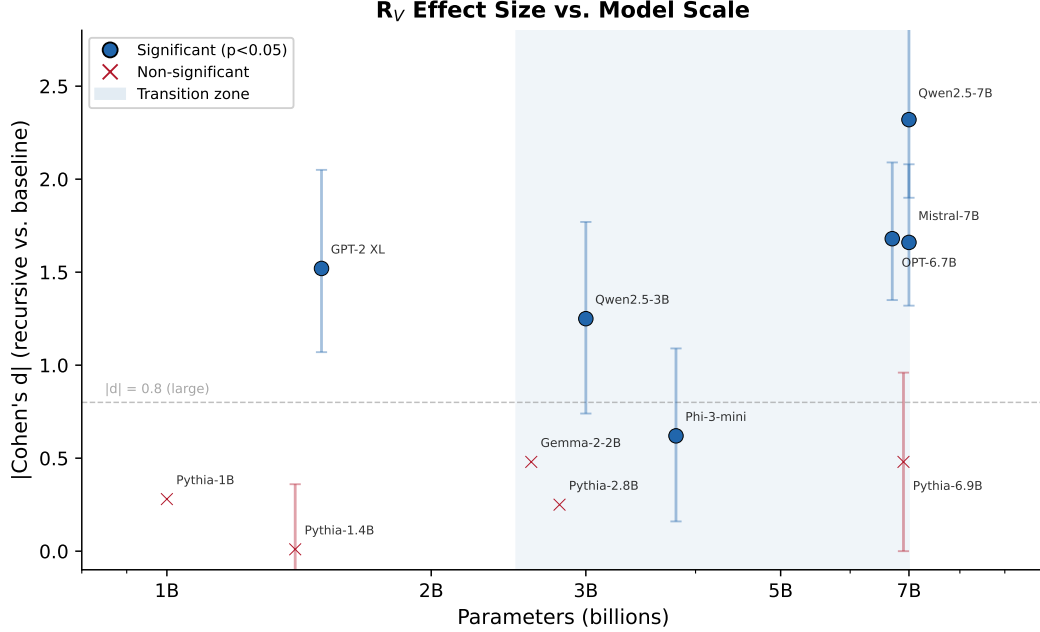
Figure 10: R_V effect size vs. model scale across 11 models. Significant effects (○) cluster above 3B parameters. Transition zone (shaded) spans 2.5–7B.
