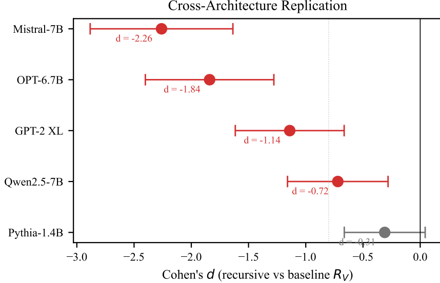
Figure 3: Cross-architecture forest plot. Signed Cohen’s d with 95% CIs for recursive vs. baseline R_V . Negative d : contraction; positive d : expansion. Dashed line: |d|=0.8 (large effect threshold).
