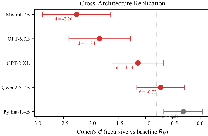
Figure 3: Cross-architecture effect sizes. Locked GQA rows contract ( d < 0 ). Two MHA architectures show pipeline-dependent sign reversal. Pythia-1.4B is null.
