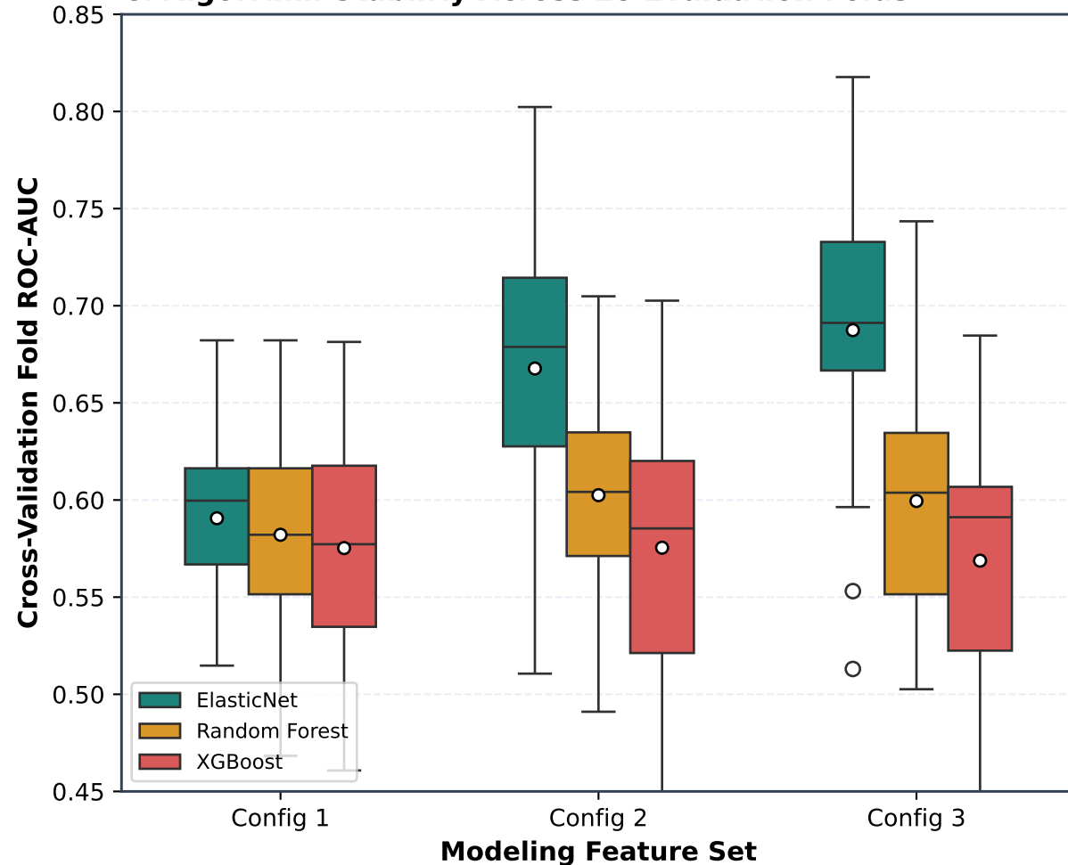
C. Algorithm Stability Across 25 Evaluation Folds
