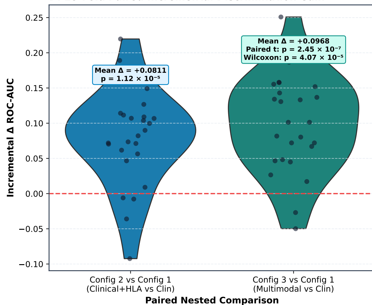
D. 25-Fold Paired Incremental Discrimination Gain
