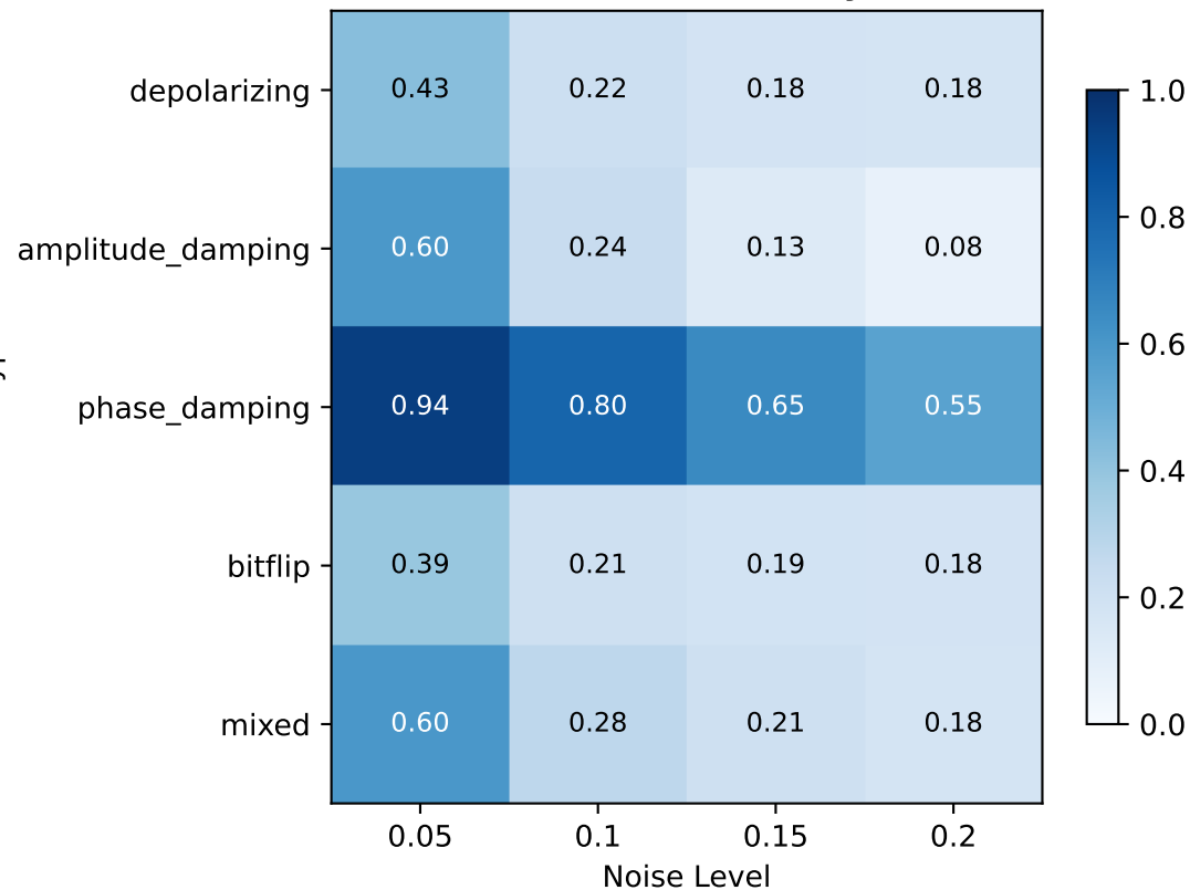
Frobenius Fidelity
