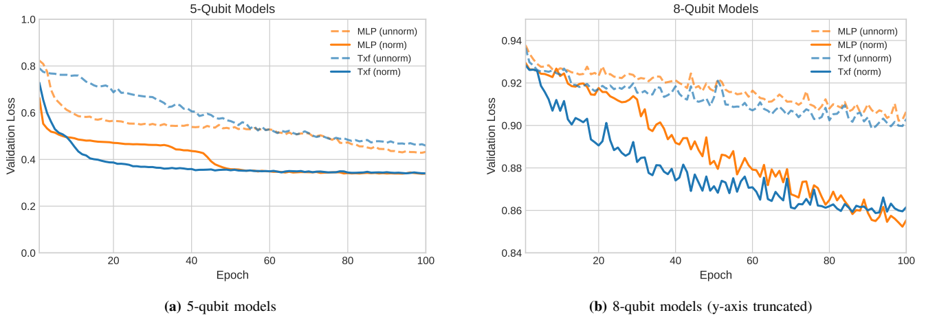
Fig. 4: Validation loss curves for unnormalized (dashed) and normalized (solid) models. (a) 5-qubit models show a clear separation between normalized and unnormalized training. (b) 8-qubit models reveal that normalized models steadily improve while unnormalized models plateau.
