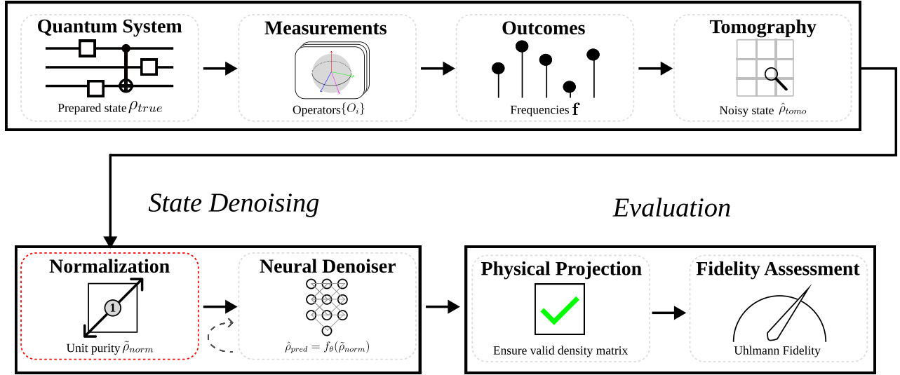
Fig. 1: Overview of the training and evaluation pipeline. Quantum states are measured, reconstructed via tomography, and normalized to unit Frobenius norm. A neural denoiser maps the normalized noisy state to a denoised estimate, which is then projected to a valid density matrix before computing Uhlmann fidelity.
