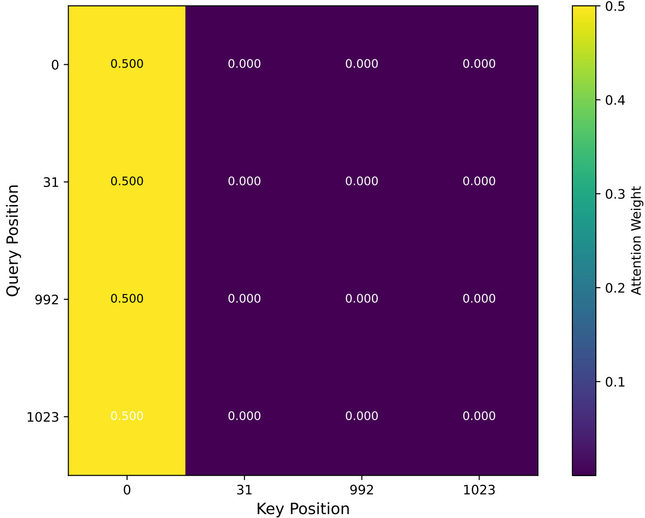
Attention Between GHZ-Correlated Elements
