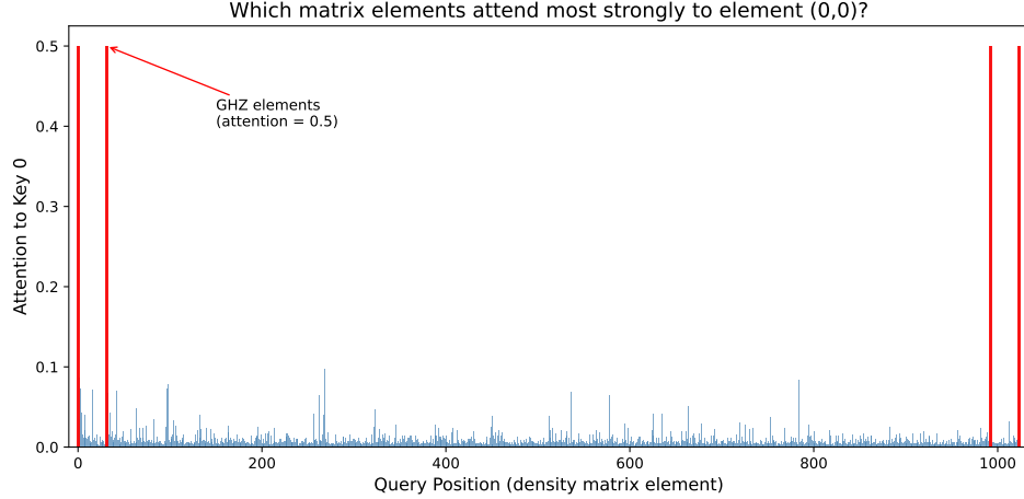
Figure 4: Attention to token 0 (the \rho_{00,00} matrix element) from all 1024 tokens. The four tall red bars at positions 0, 31, 992, and 1023 correspond exactly to the GHZ state’s non-zero elements—the model learns that these specific elements should attend strongly to each other (attention weight 0.5, versus mean 0.01 for other elements).
