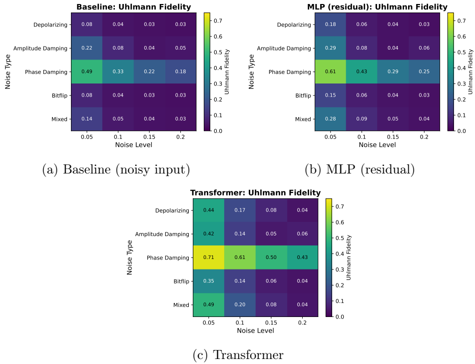
Figure 3: Uhlmann fidelity by noise type and level. Rows: noise channels; columns: noise strength p \in \{0.05, 0.10, 0.15, 0.20\} .
