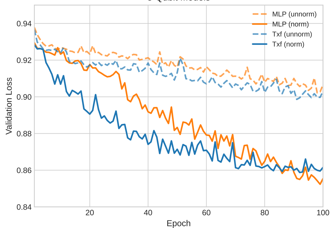
8-Qubit Models
