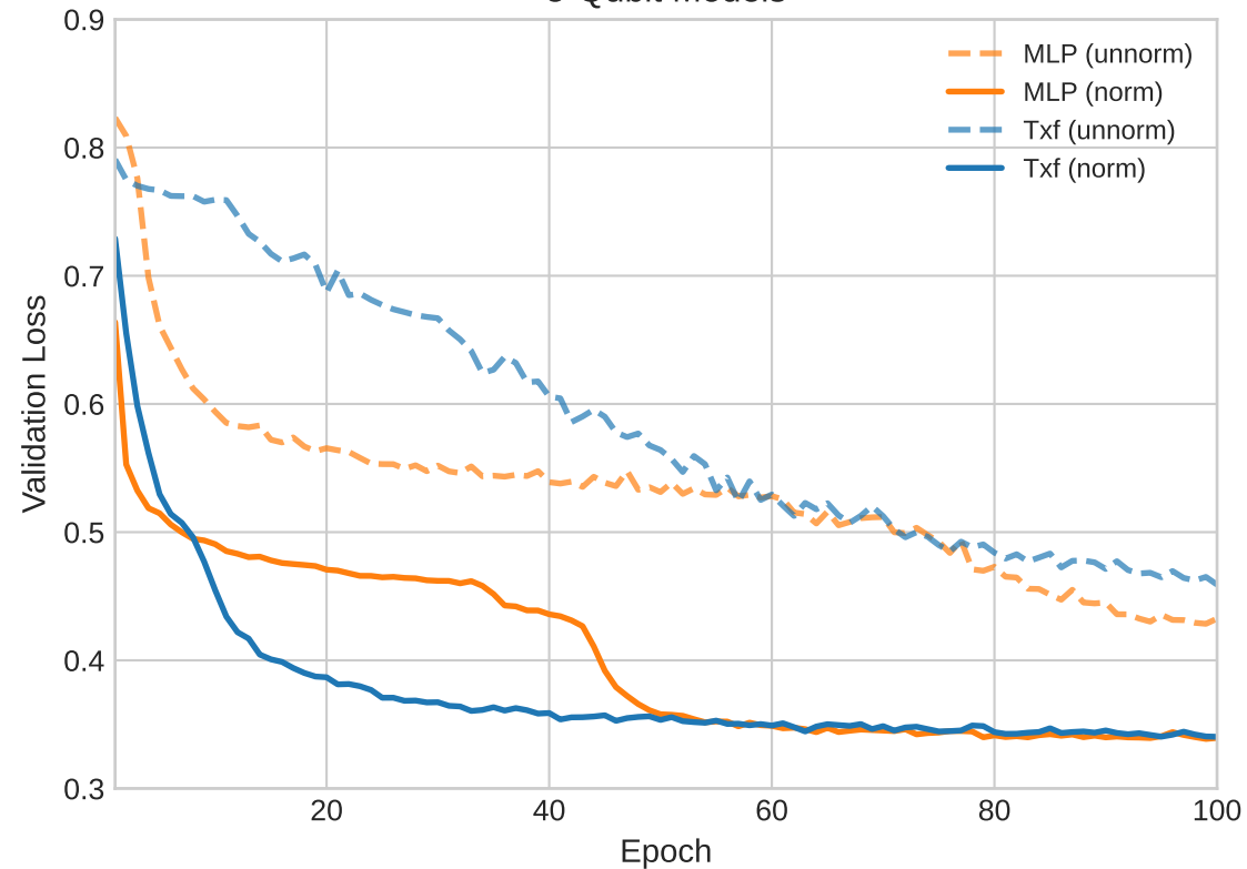
5-Qubit Models
