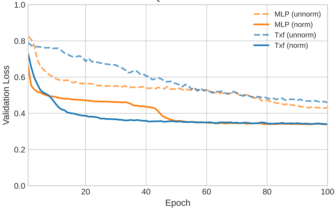
5-Qubit Models
