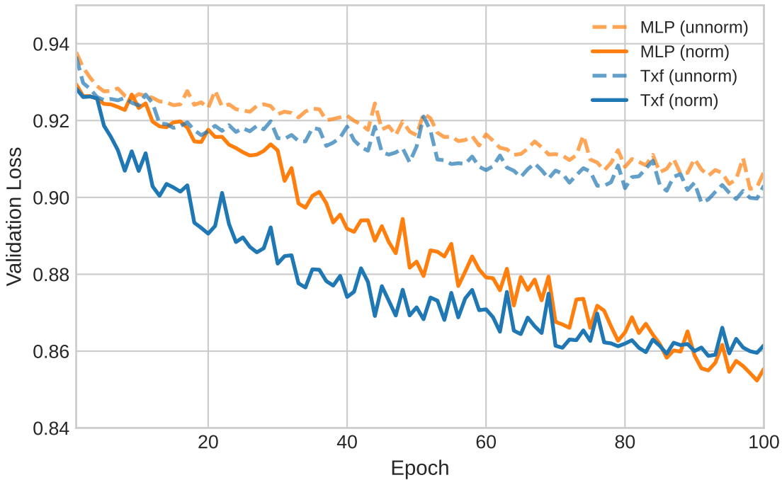
8-Qubit Models
