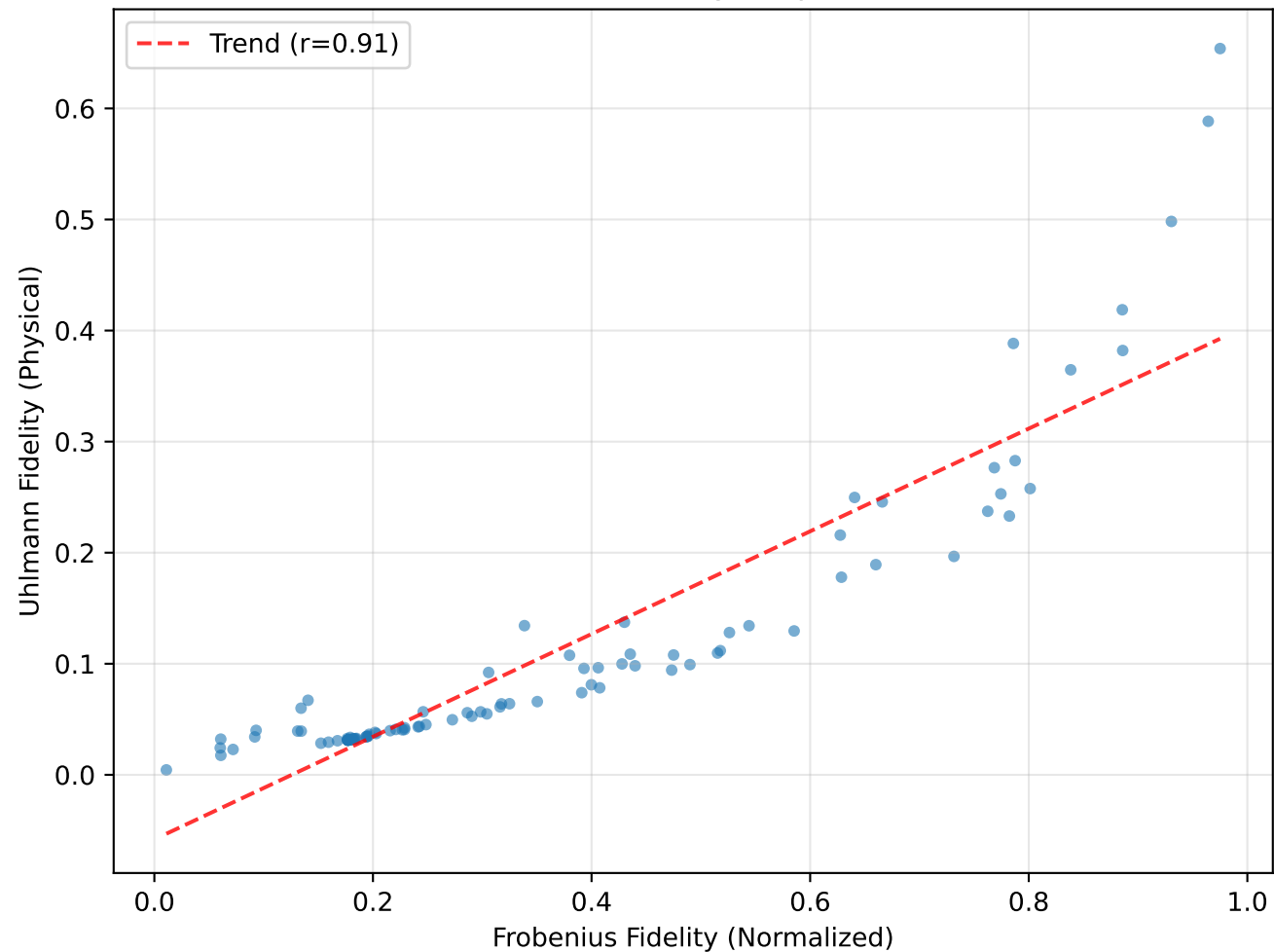
Frobenius vs Uhlmann Fidelity (5-qubit subset, N=100)
