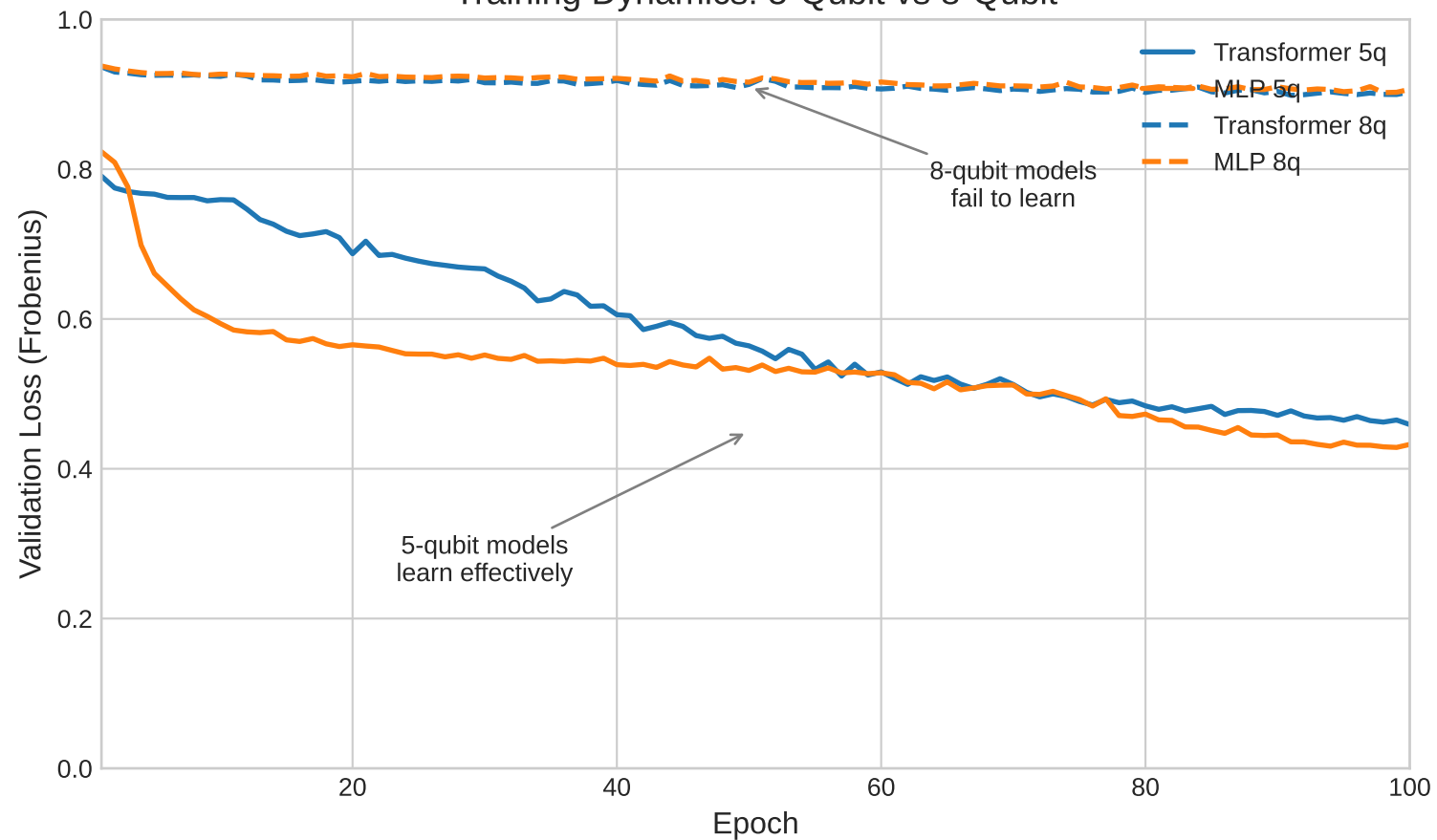
Training Dynamics: 5-Qubit vs 8-Qubit
