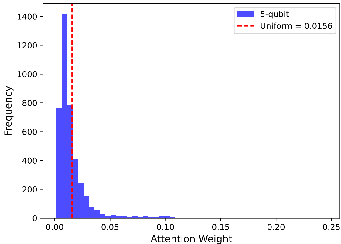
5-Qubit Attention Distribution
