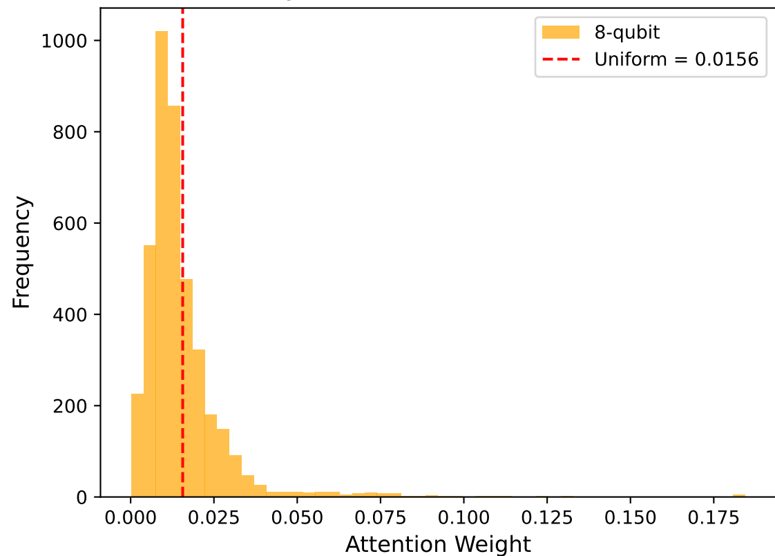
8-Qubit Attention Distribution
