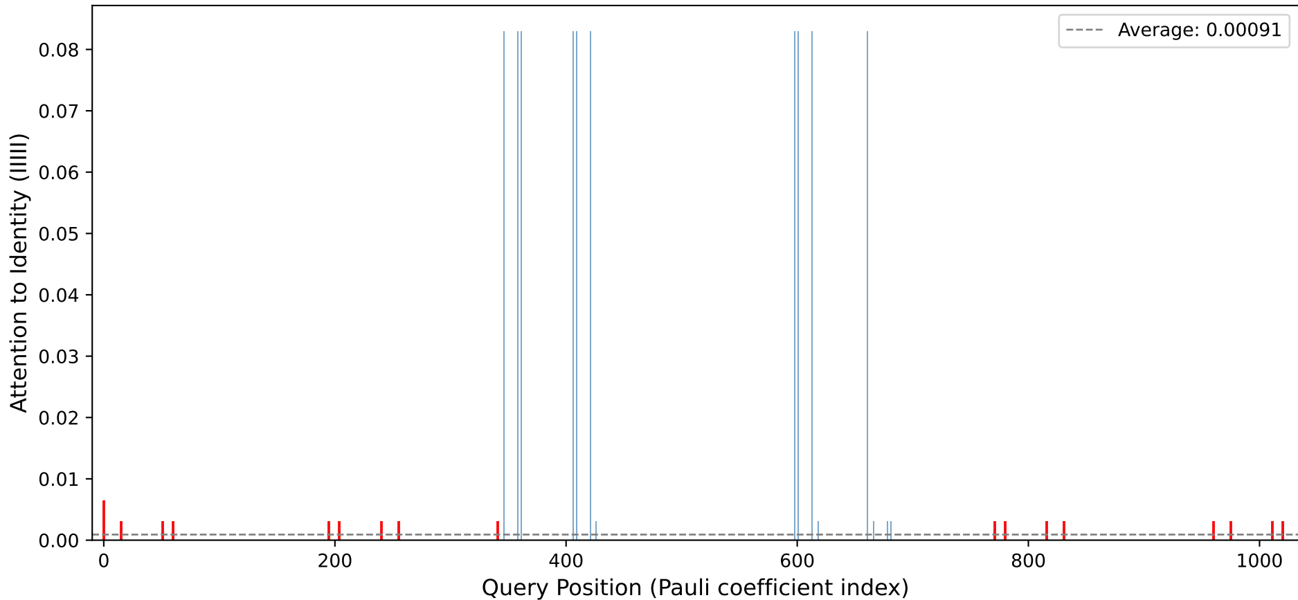
Pauli Transformer: Attention to Identity Coefficient
