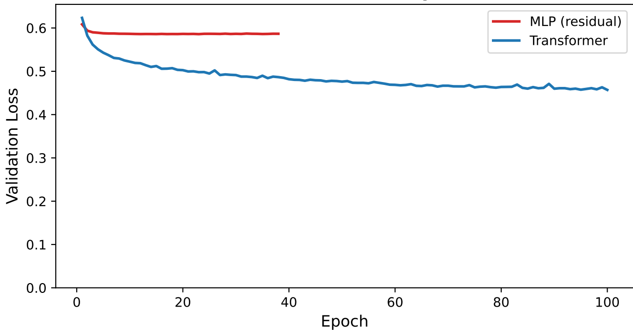
Validation Loss vs Epoch
