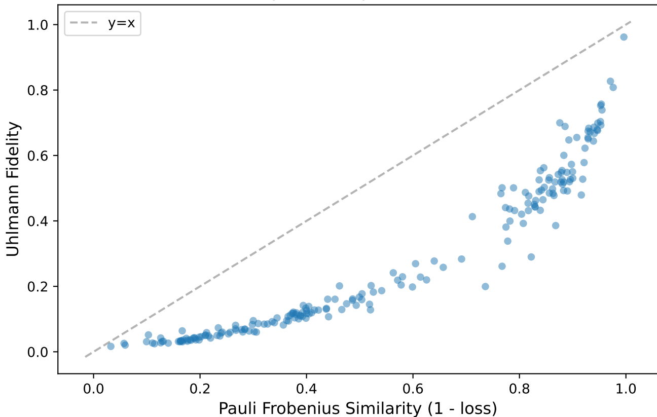
Pauli Frobenius vs Uhlmann Fidelity (Spearman \rho = 0.986 )
