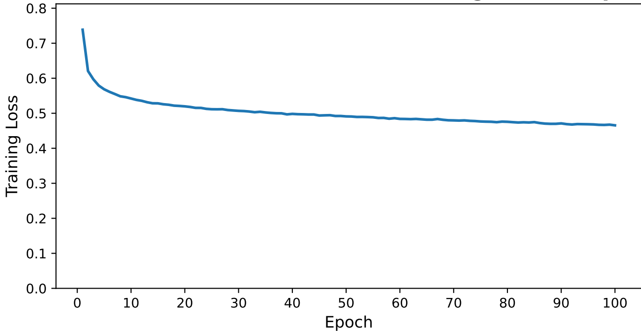
Transformer-Small Frobenius Training Loss vs Epoch
