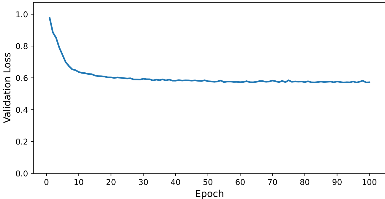
Transformer-Small Physics Validation Loss vs Epoch
