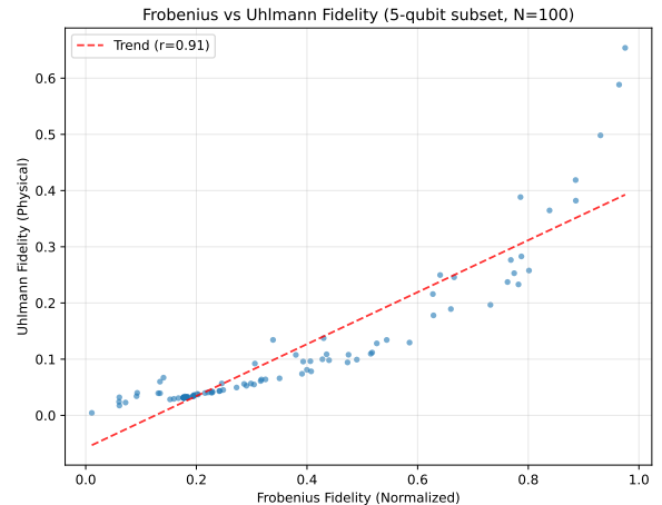
Fig. 3: Correlation between Frobenius fidelity (normalized) and Uhlmann fidelity (physical) on a random subset of the 5-qubit dataset. The strong correlation ( r = 0.91 ) justifies using Frobenius fidelity as a training proxy.
