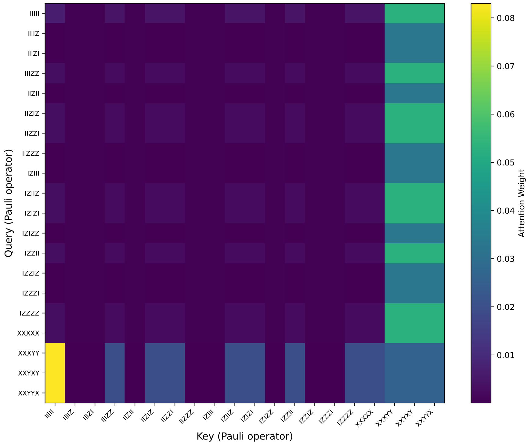
Attention Between GHZ-Relevant Pauli Coefficients
