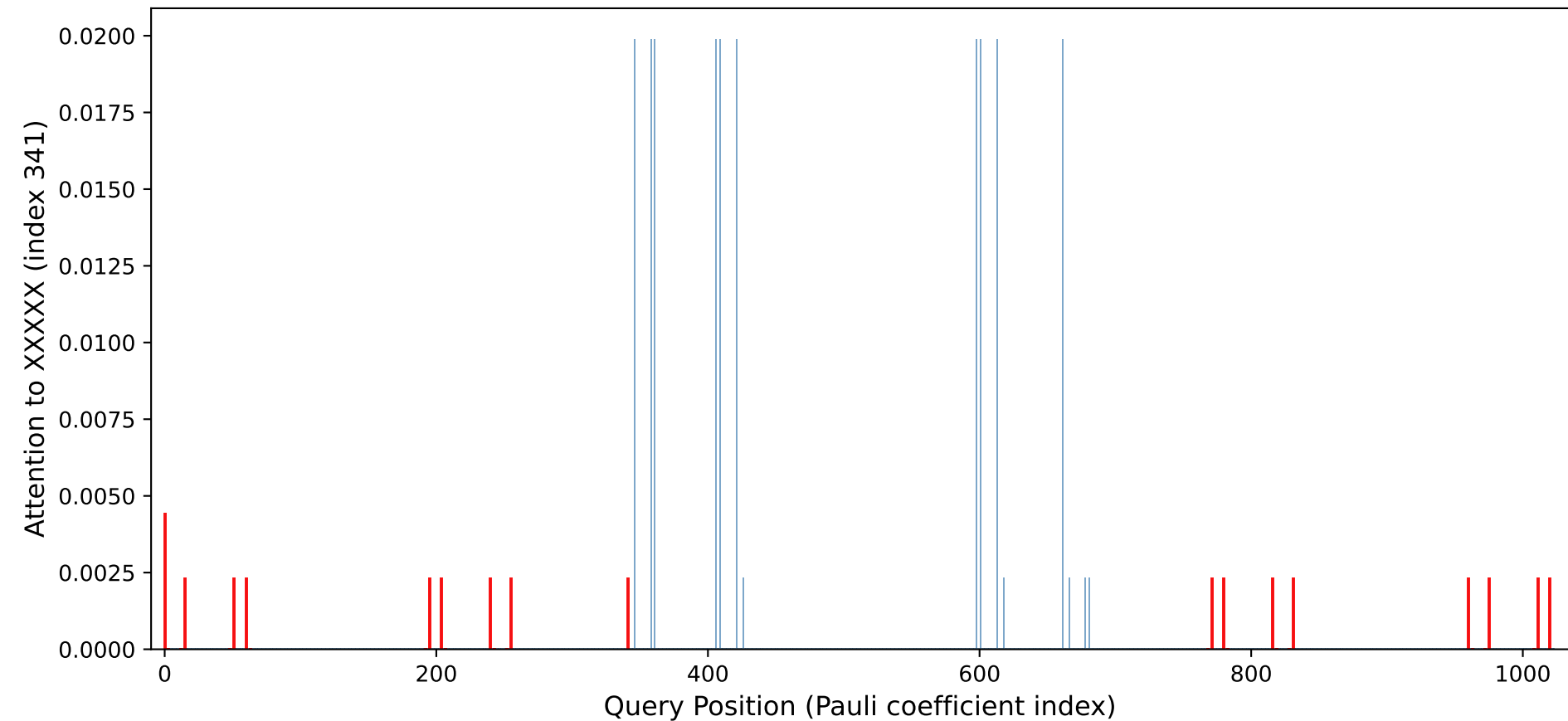
Pauli Transformer: Attention to XXXXX Coefficient
