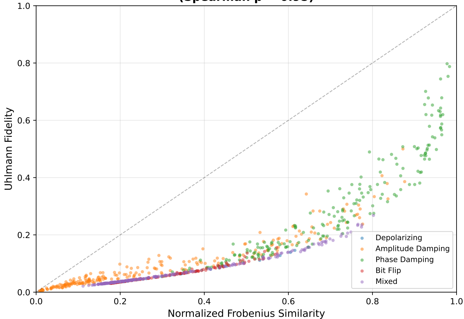
Frobenius Similarity vs Uhlmann Fidelity (Spearman \rho = 0.95 )
