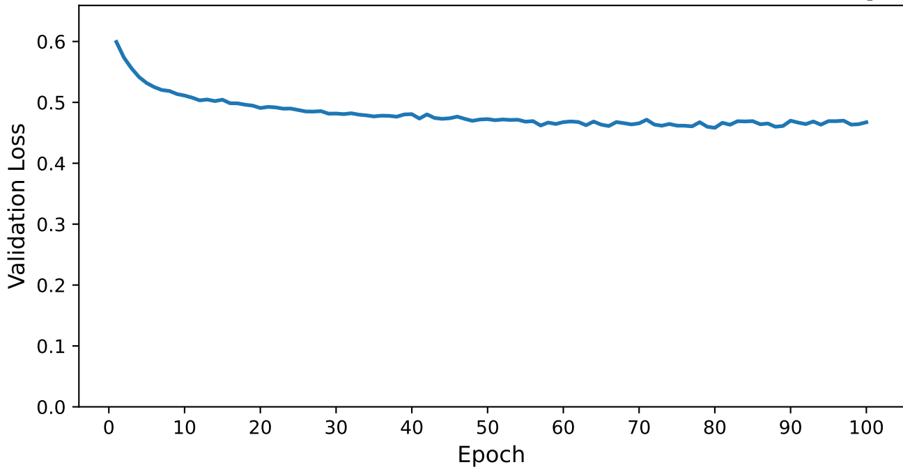
Transformer-Small Frobenius Validation Loss vs Epoch
