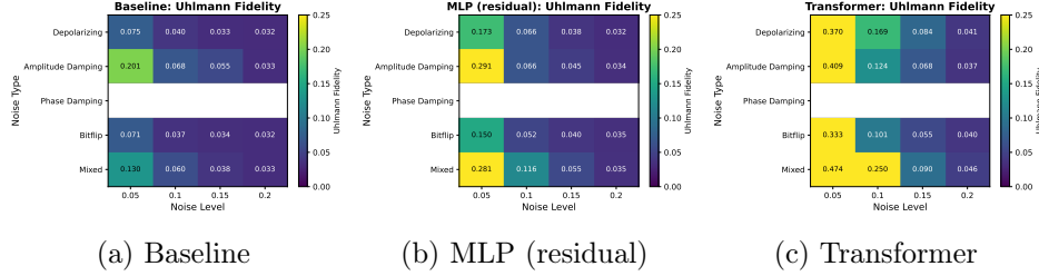
Figure 2: Uhlmann fidelity by noise type and level. The Transformer achieves higher fidelity across all conditions, with the largest improvements on amplitude damping and mixed noise.
