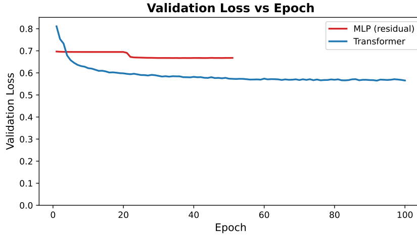
Figure 1: Validation loss during training. The Transformer converges rapidly to a lower loss, while the MLP plateaus at a higher value despite the residual architecture.
