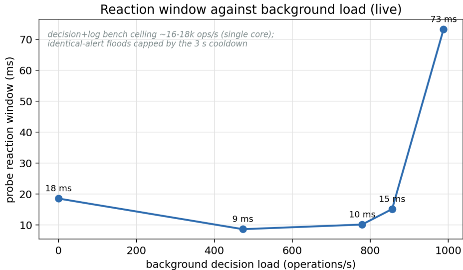
Figure A.16: Reaction window against background decision load on the live testbed: the window holds in the tens of milliseconds up to about a thousand operations a second, rising only as the single-threaded controller nears the decision-and-log bench ceiling of sixteen to eighteen thousand a second. Source: results/gap1.live/curve.csv .
